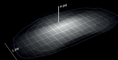
LA-01 Asimmetrica stradale / Street asymmetrical L / H = 1,25
